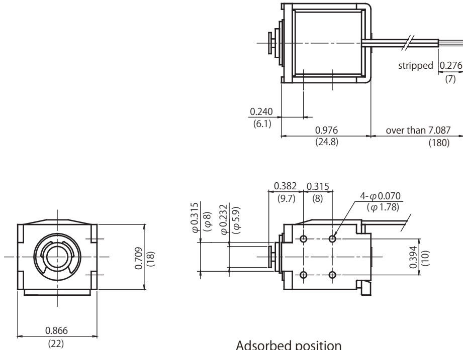
Adsorbed position
