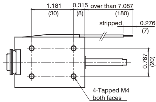
Adsorbed position
